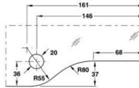
Cut Out for DPF-30
