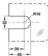
Cut Out for DPL-3A
