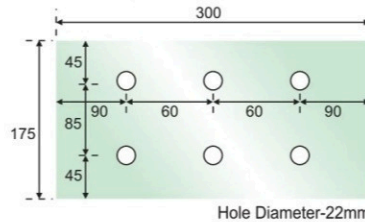
DSP-300 Splice Plate 300mm
