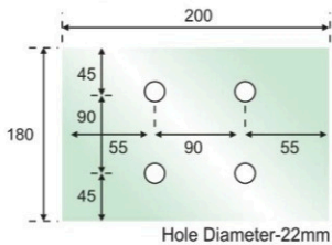
DSP-200 Splice Plate 200mm
