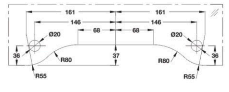
Cut Out for DPF-61
