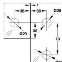
Cut Out for DVPF-610 ST
