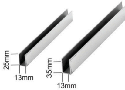
DGPL-2 'U' Channel (For Fixed Glass) Finish: CP/ SS Available in 3.4 Mtr., Thickness: 1.5mm
