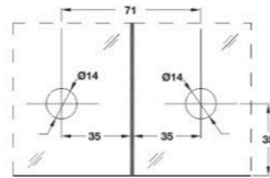
Cut Out for DPF-630
