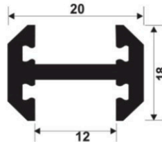
DGP-114 Glass Edge Profile for Partition (Black Matt)
