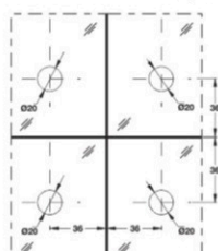
Cut Out for DPF-620 (F)
