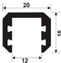
DGP-113 Glass Edge Profile (Black Matt)
