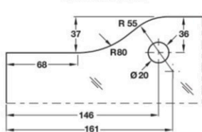
Cut Out for DPL-2A
