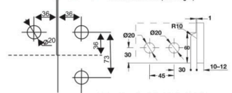
Cut Out for DPF-610 (L/R)
