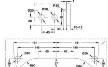
Cut Out for DPF-51
