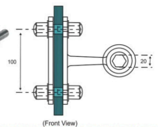
DSP-A22 1 Way Spider for Wall/Ceiling
