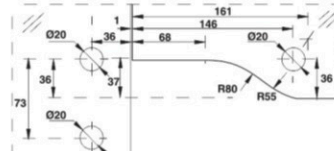
Cut Out for DPF-41 (L) & DPF-41 (R)
