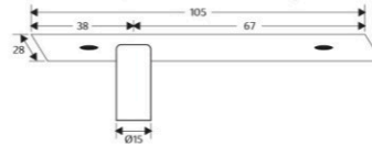
Cut Out for DFS-ACC-GDP
