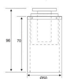
DSA-01 Iron Assembly
