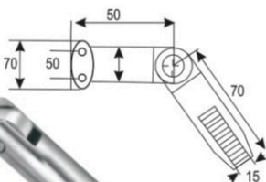
DCF-3 Wall to Rod Connector
