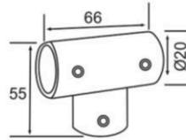
DKH-3 (Brass) Rod to Rod (Dia 19mm)
