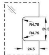
Cut Out for DPL-3B
