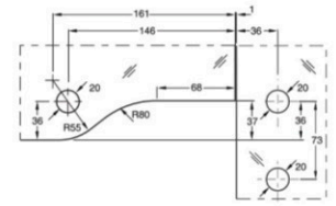
Cut Out for DPF-40
