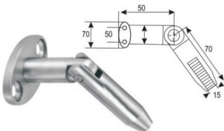
DCF-3 Wall to Rod Connector
